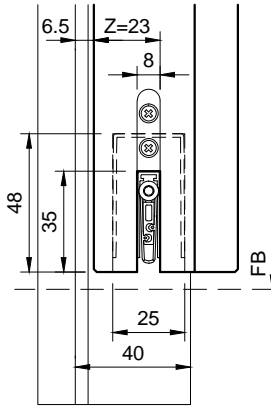
Typ: RD17-40 49-61mm Türblatt
