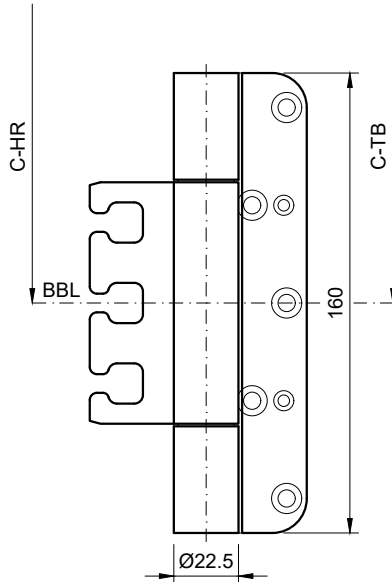
VX7939/FD/160 18/5 (HR) Edelstahl matt
